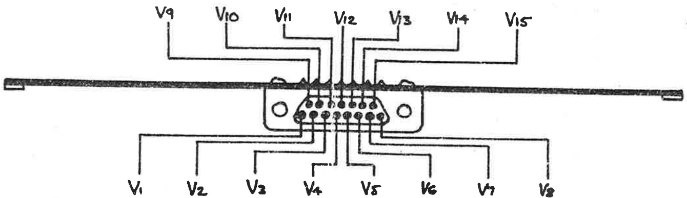
DB-15 CONNECTOR. PIN SCHEMATIC (RIGHT ANGLE-FEMALE)
